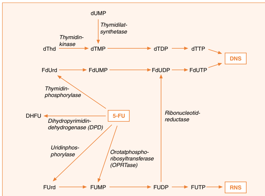
Abb. 1. Metabolismus und Katabolismus von Fluorouracil [nach 1] dTMP: Desoxythymidinmonophosphat, dTDP: Desoxythymidindiphosphat, dTTP: Desoxythymidintriphosphat, dUMP: Desoxyuridinmonophosphat, 5-FU: 5-Fluorouracil, FdUrd: 5-Fluoro-2'-desoxyuridin, FdUMP: 5-Fluoro-2'-desoxyuridinmonophosphat, FdUDP: 5-Fluoro-2'-desoxyuridindiphosphat, FdUTP: 5-Fluoro-2'-desoxyuridintriphosphat, FUrUrd: 5-Fluorouridin, FUMP: 5-Fluorouridinmonophosphat, FUDP: 5-Fluorouridindiphosphat, FUTP: 5-Fluorouridintriphosphat, DHFU: Dihydrofluorouracil
